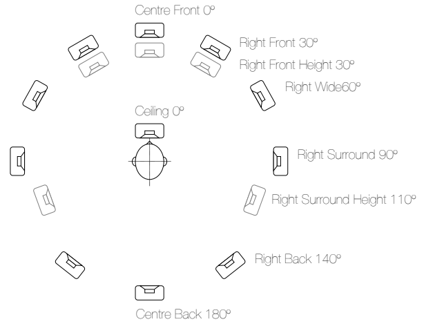
Figure 4.4: Loudspeaker positions associated with the speaker roles available in the television. The True Image processor delivers a unique output to each of these output channels.
