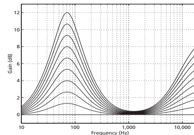
Figure 3.5: An example of the effect of the Loudness on the Magnitude response of the system at different volume settings. The lowest curve is for a high volume setting. The highest curve represents the response at a low volume setting. In this example, the Bass Max Boost is set to 12 dB and the Treble Max Boost is set to 9 dB.
