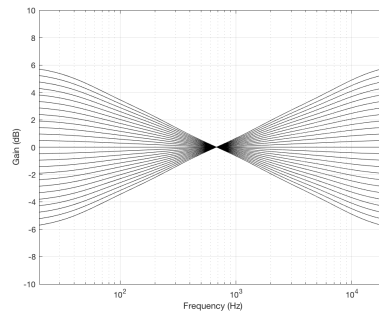
Figure 3.3: Magnitude response measurements of all settings of the Frequency Tilt control. Note that this response is applied to each input channel.
