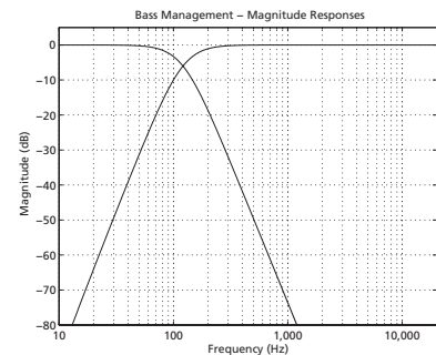
Figure 3.7: Magnitude response of the crossover used in the Bass Management system, showing an example with default frequency of 120 Hz.
