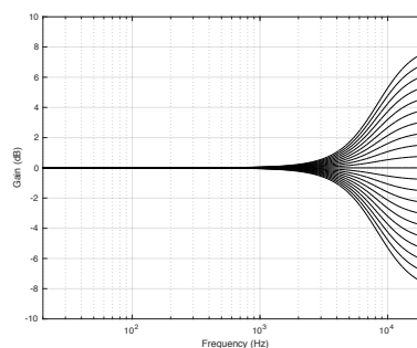
Figure 3.2: Magnitude response measurements of all settings of the Treble control. Note that this response is applied to each input channel.
