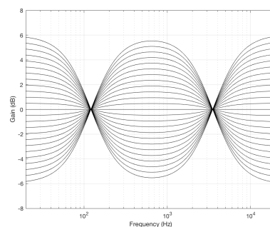
Figure 3.4: Magnitude response measurements of all settings of the Sound Enhance control. Note that this response is applied to each input channel.
