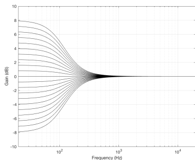
Figure 3.1: Magnitude response measurements of all settings of the Bass control. Note that this response is applied to each input channel.
